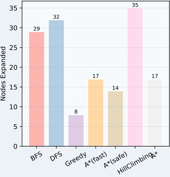
Nodes Expanded by Algorithm
